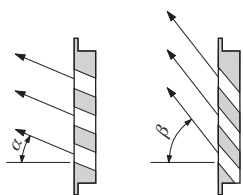
Jet bundle elements with different discharge angles
