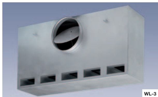
Figure 2: Linear whirl outlet with connection box and connection spigot;
