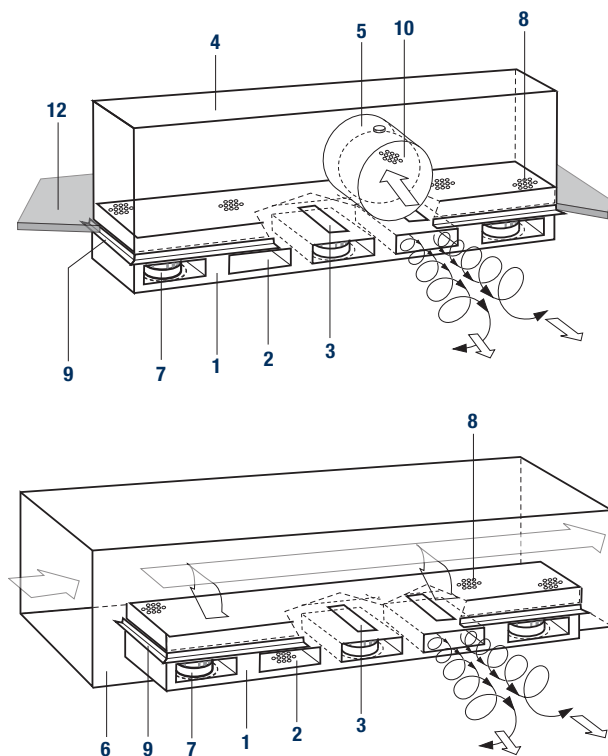
Figure 1: Linear whirl outlet
